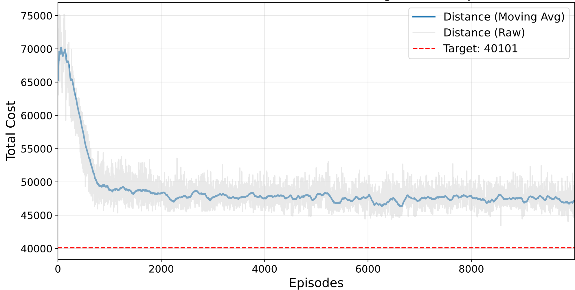
Final Masked AutoRL-SOP Training - ft70.2.sop
